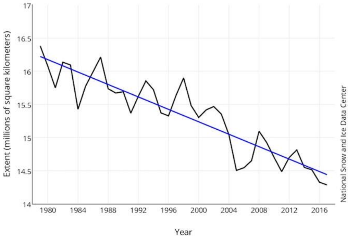
Average Monthly Arctic Sea Ice Extent February 1979 - 2017
